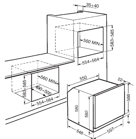
Technical drawing for ovens with codes beginning: SF750, SFP750 & SF700
