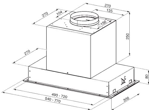
KSEG54X-1 54cm canopy hood
