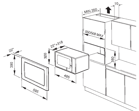
FME120 Silver glass Coordinates with "Linea" aesthetic
