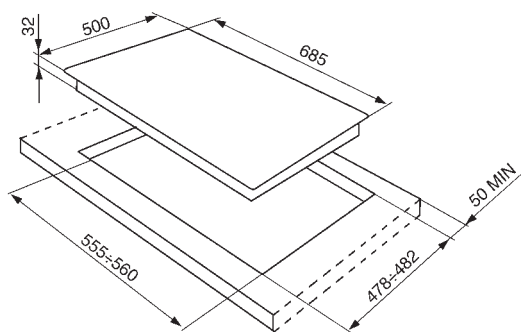
Technical drawing for all 70cm hobs
