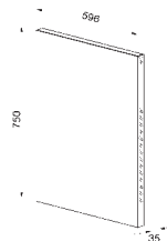
SY62MX8 - Splashback KITC6X SY6CPX8 - Splashback KITC6X
